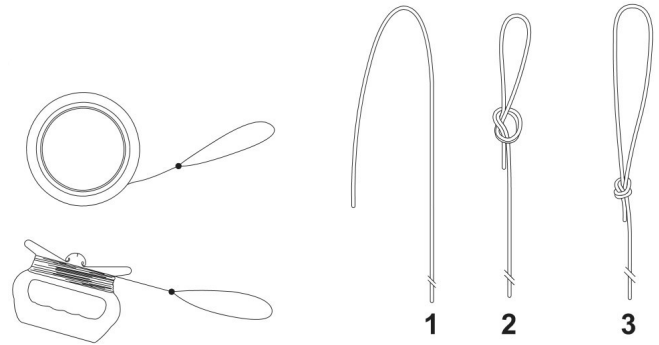
FIGURE 2. ATTACH THE LINE TO THE KITE
